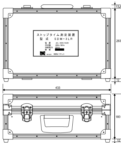
測定器本体 / Measuring Instrument Model: SDM-3LR
